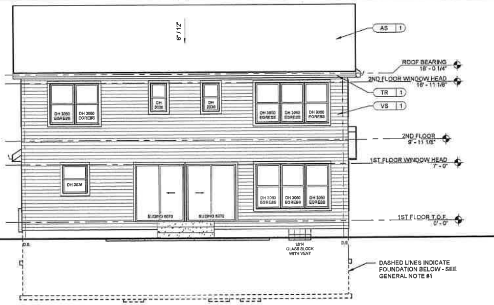
4 REAR ELEVATION SCALE: 3/16" = 1'-0"
