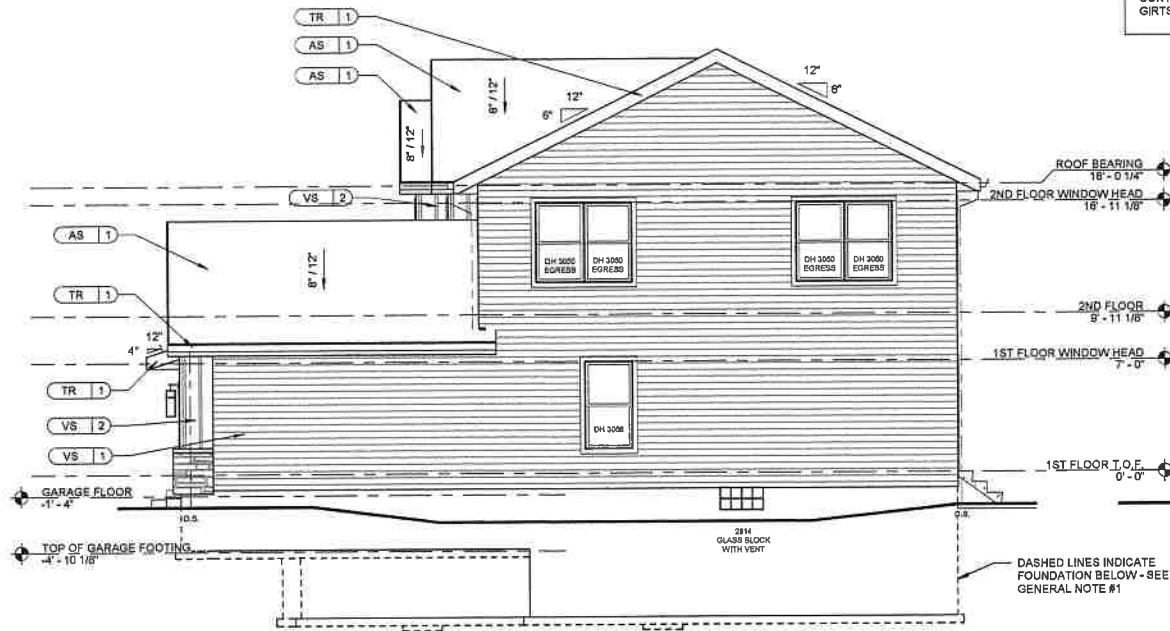
3 RIGHT ELEVATION SCALE: 3/16" = 1'-0"
