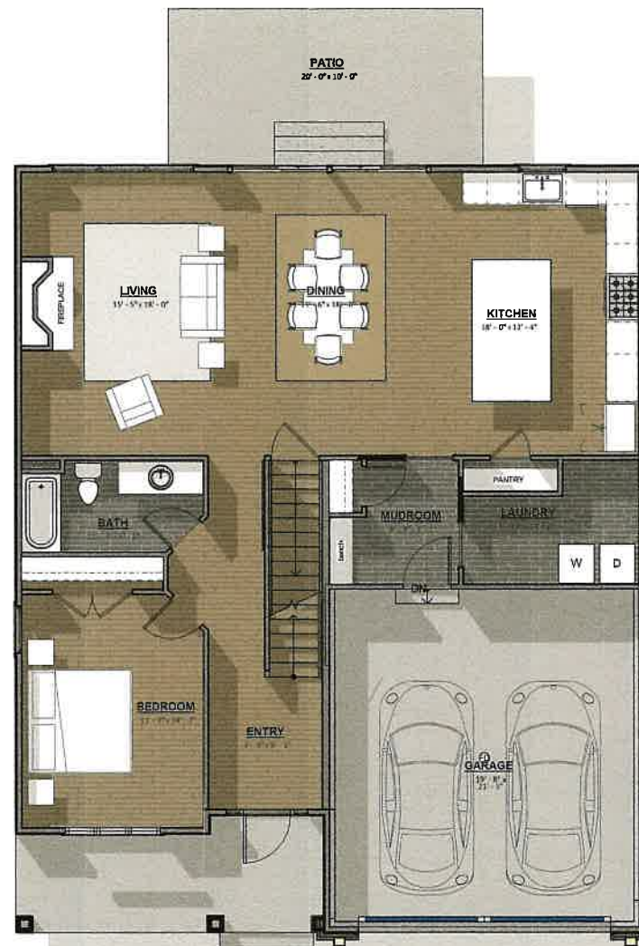
FIRST FLOOR +/- 1,400 SF (+/- 440 SF GARAGE)
