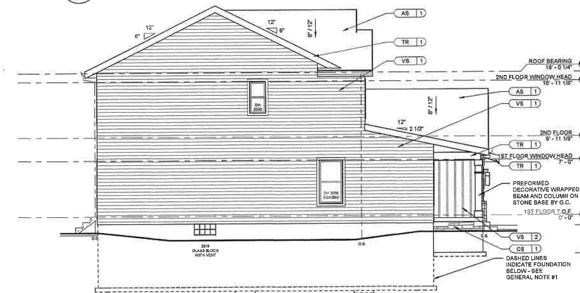
2 LEFT ELEVATION SCALE: 3/16" = 1'-0"
